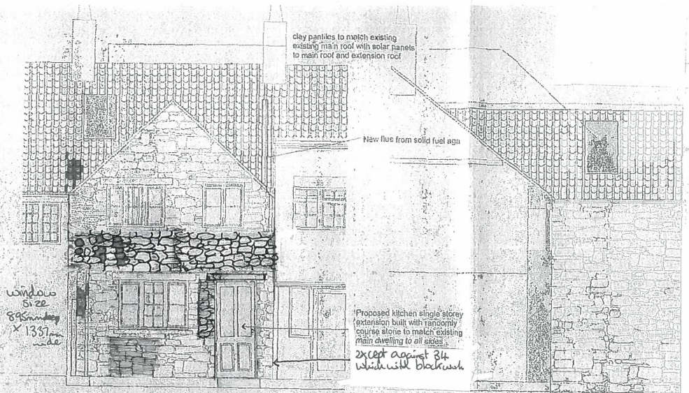
PROPOSED REAR ELEVATION 1:50
